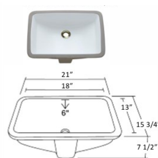
1813 (Large Rectangle)
